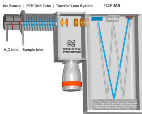
Figure 1 Schematic drawing of a PTR-TOF-MS.
